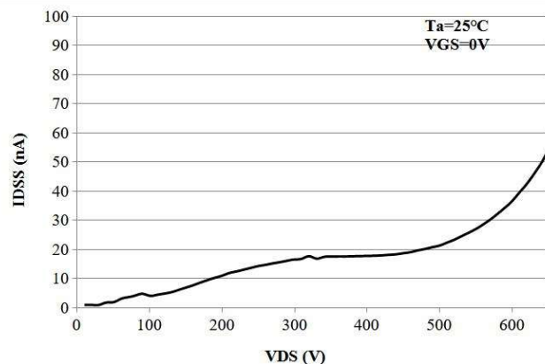
Breakdown voltage @ T_j = 25^\circ\text{C} , V_{GS} = 0\text{V}
