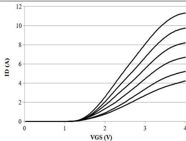
I_{DS} vs. V_{GS} @ T_j = 25^\circ\text{C}-150^\circ\text{C} , step 25^\circ\text{C}
