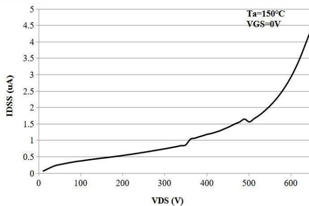
Breakdown voltage @ T_j = 150^\circ\text{C} , V_{GS} = 0\text{V}
