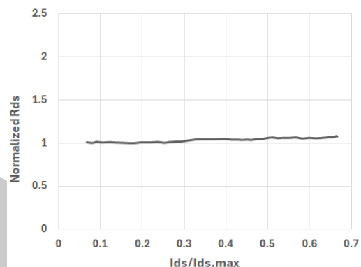
Normalized R_{DS(on)} vs. I_{DS}
