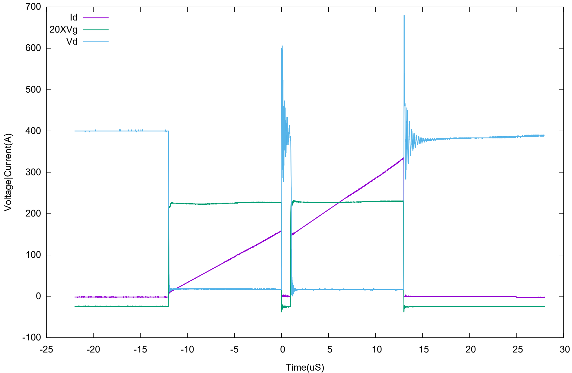
Bluesky120 (Rgon/off=2/0 Ohm); Id smoothed for clarity
