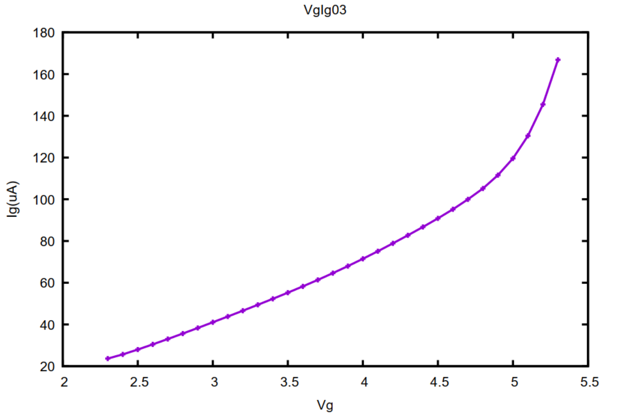
Gate leakage @ V_{ds}=0.1 V, V_s=V_b=GND
