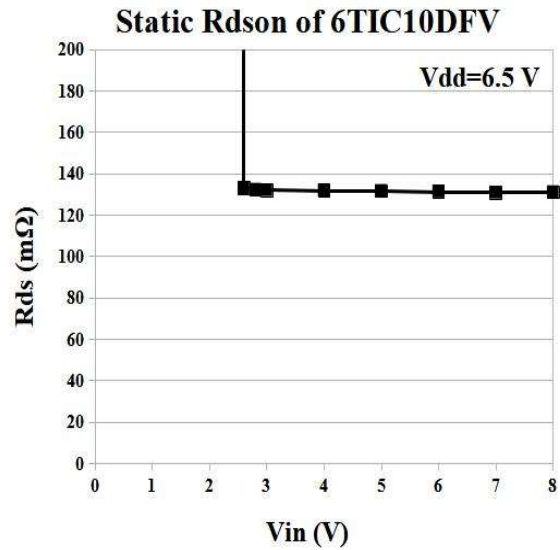
Static R ds(on) vs V in @V dd =6.5V
