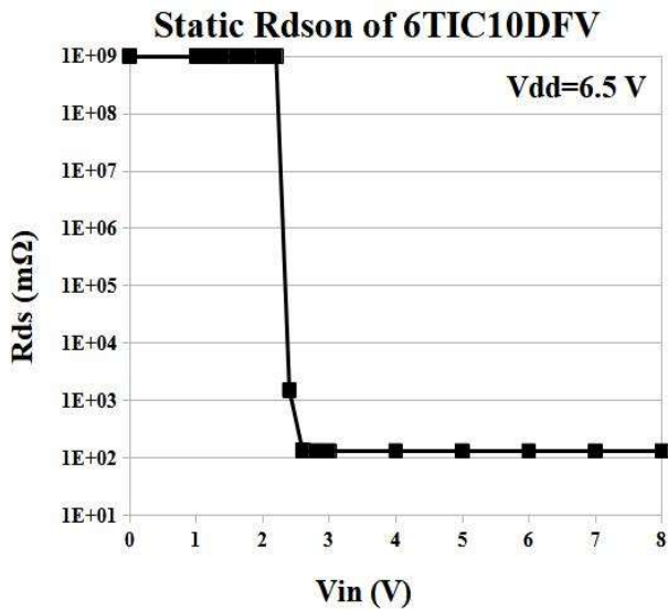
Static R ds(on) vs V in @V dd =6.5V
