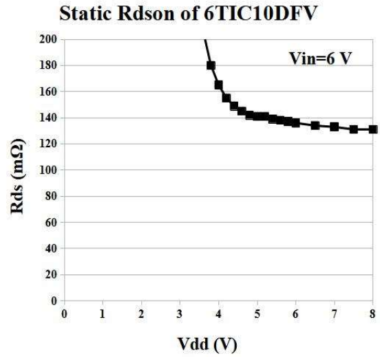
Static R ds(on) vs V dd @V in =6V
