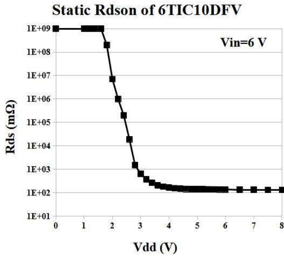
Static R ds(on) vs V dd @V in =6V
